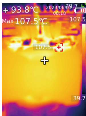
Thermal image of main transformer
