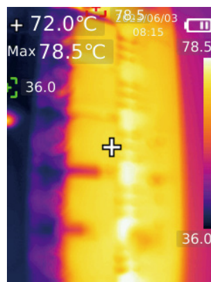
Thermal image of front-end MOSFET
