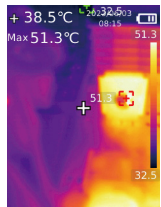
Thermal image of back-end IGBT
