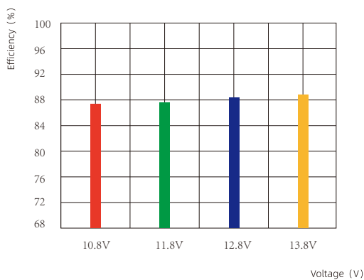
Efficiency Comparison of Full Load Power Output (3080W) at Different Input Voltages
